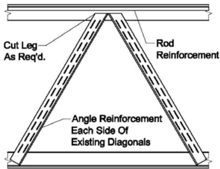
Figure 3.10 Angle Reinforcement on Rod Web Joist
