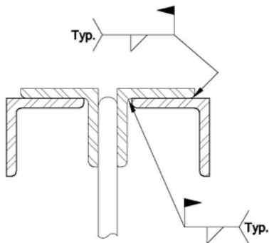
Figure 3.3 Top Chord Reinforcement – Angles
