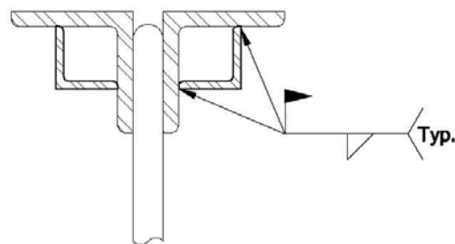
Figure 3.4 Top Chord Reinforcement - Angles
