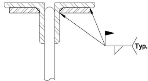
Figure 3.2 Top Chord Reinforcement - Plates
