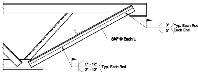
Figure 3.40 Reinforcing of End Diagonals
