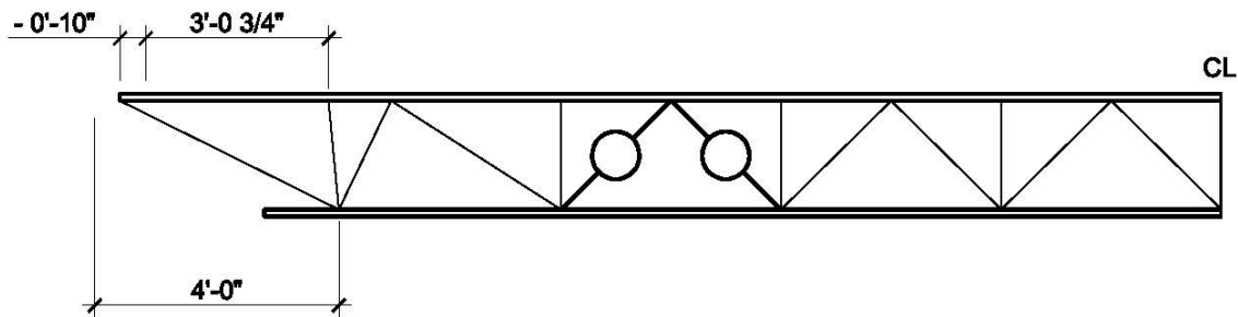
Figure 4.1 Joist to be Shortened
