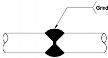
Figure 3.8 Rod Splice
