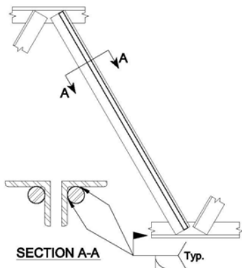
Figure 3.19 Rod Reinforcing
