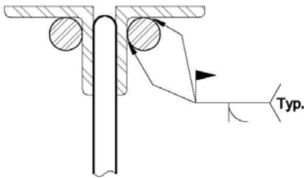
Figure 3.1 Top Chord Reinforcement – Rods
