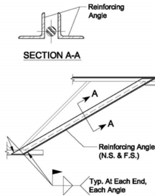
Figure 3.21 End Diagonal Reinforcing
