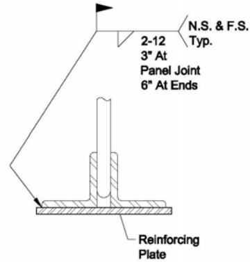
Figure 3.9 Bottom Chord Reinforcement
