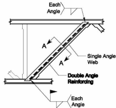
Figure 3.12 Crimped Web Reinforcement
